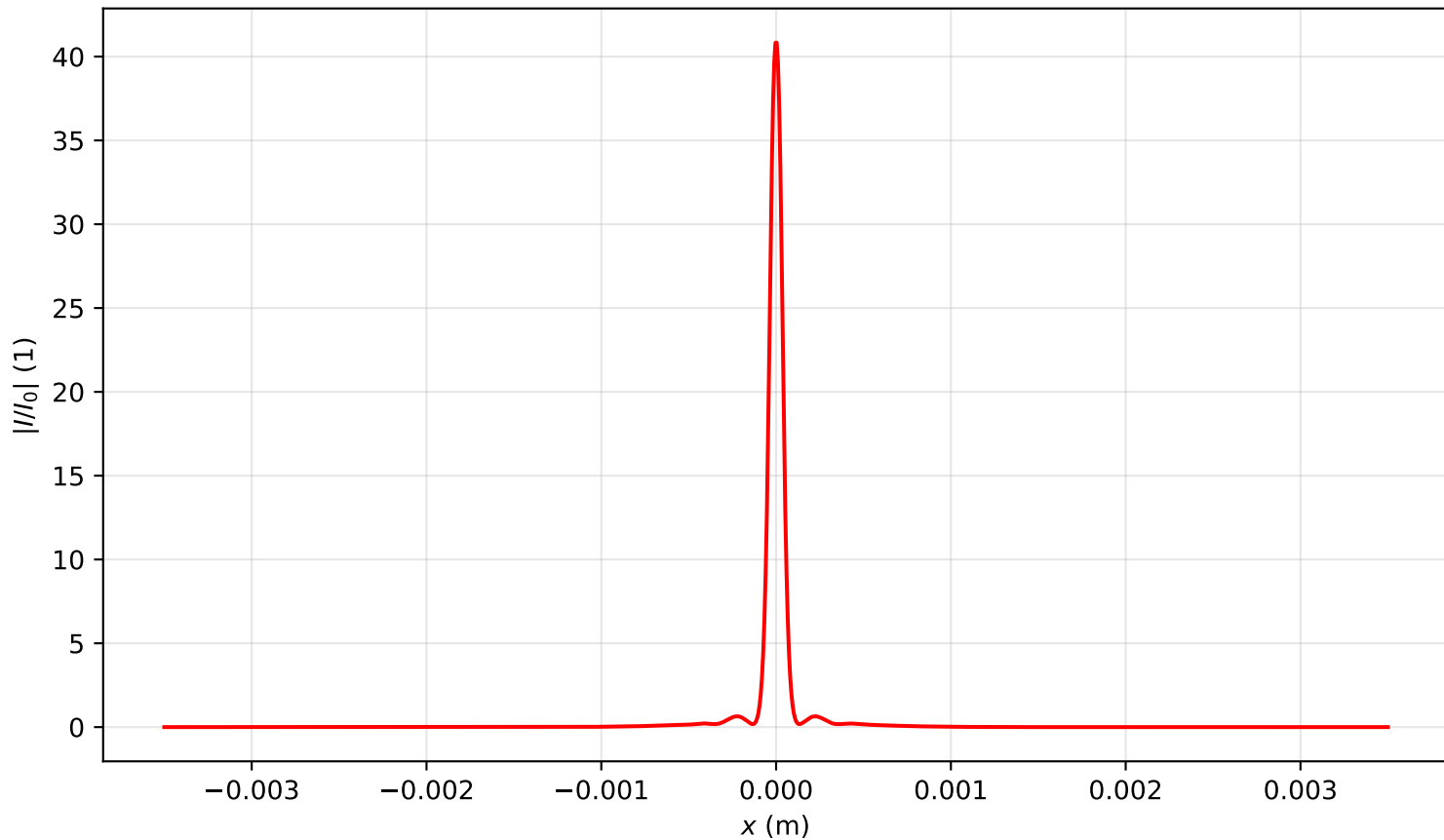
Intensity profile I(x, y = 0, z = 0.955)/I_0 , P_{in}=2.5P_{cr} , artificial time
